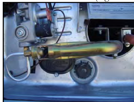
Figure 4-11. Water Heater Drain
