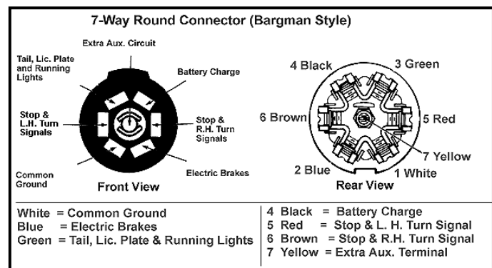
Figure 7-13. Bargman Seven-Pin Towing Connector
