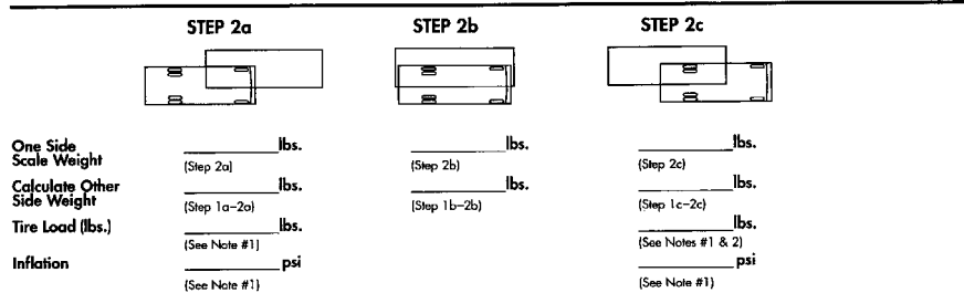
Figure 13-8. Procedure for Weighing the Motor Home (Each Tire Position Individually)
