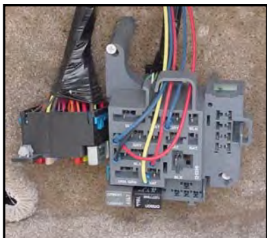
Figure 7-11. Fuse Blocks
